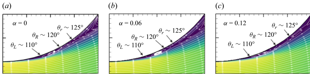
Figure 18. The PIV time-averaged velocity magnitude and streamlines on the non-seam side at Re = 1.69 \times 10^5 and the seam angle 15^\circ for varying spin rates. Separation and reattachment angles shown to nearest 5^\circ (Jackson et al. 2020) with (a) \alpha_{Jackson} = 0.0 ; (b) \alpha_{Jackson} = 0.06 ; (c) \alpha_{Jackson} = 0.12 . Yellow contours indicate high velocity, dark blue contours indicate zero velocity.
